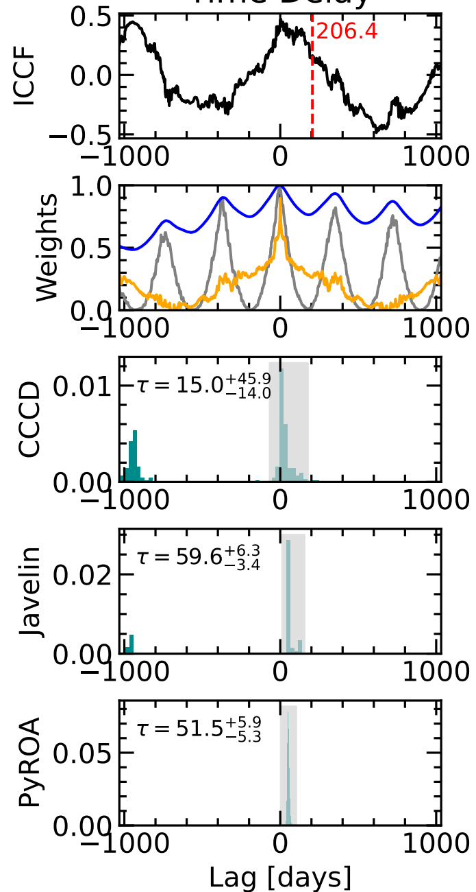
Time Delay
