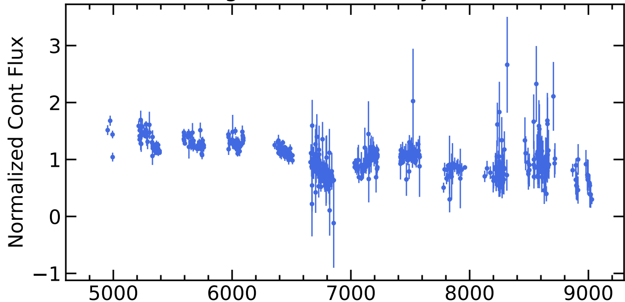
RM470 Light Curves (w/ PyROA model)
