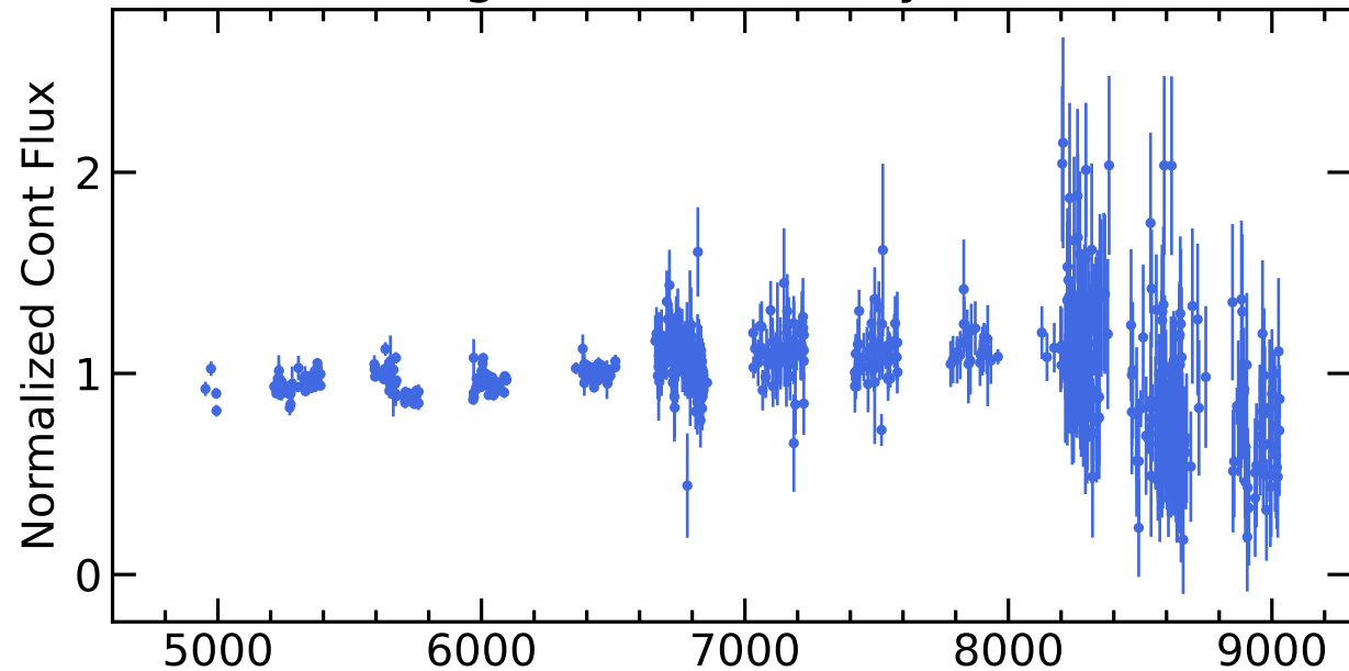
RM471 Light Curves (w/ PyROA model)
