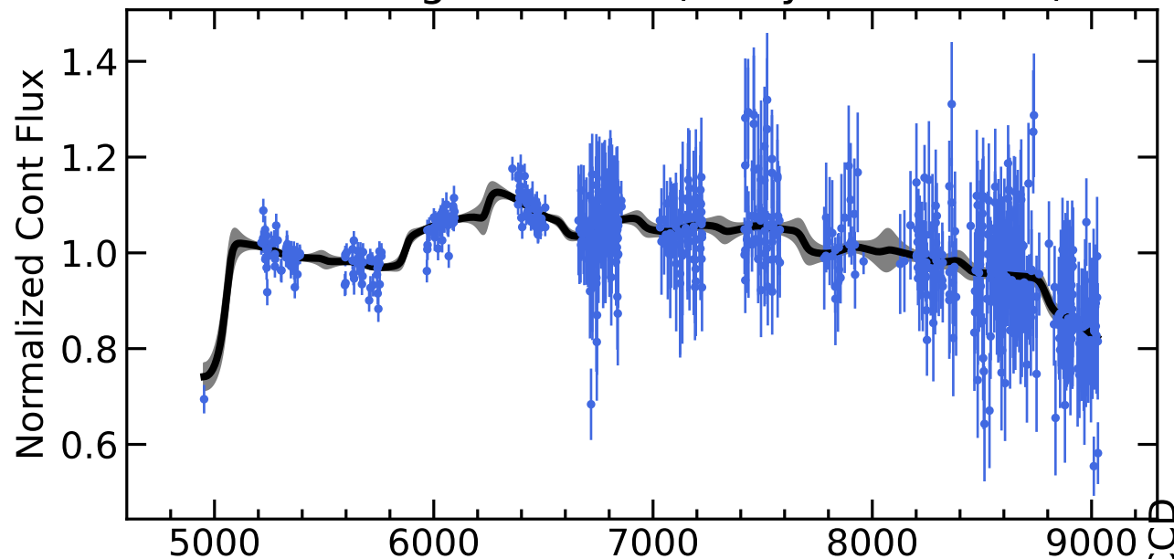
RM472 Light Curves (w/ PyROA model)
