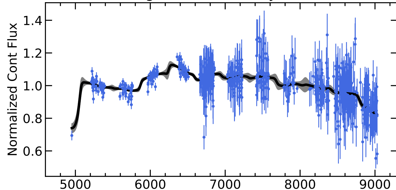
RM472 Light Curves (w/ PyROA model)
