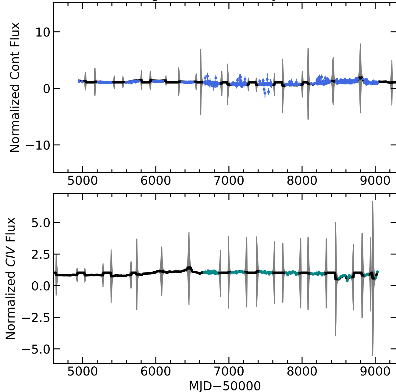
RM475 Light Curves (w/ PyROA model)
