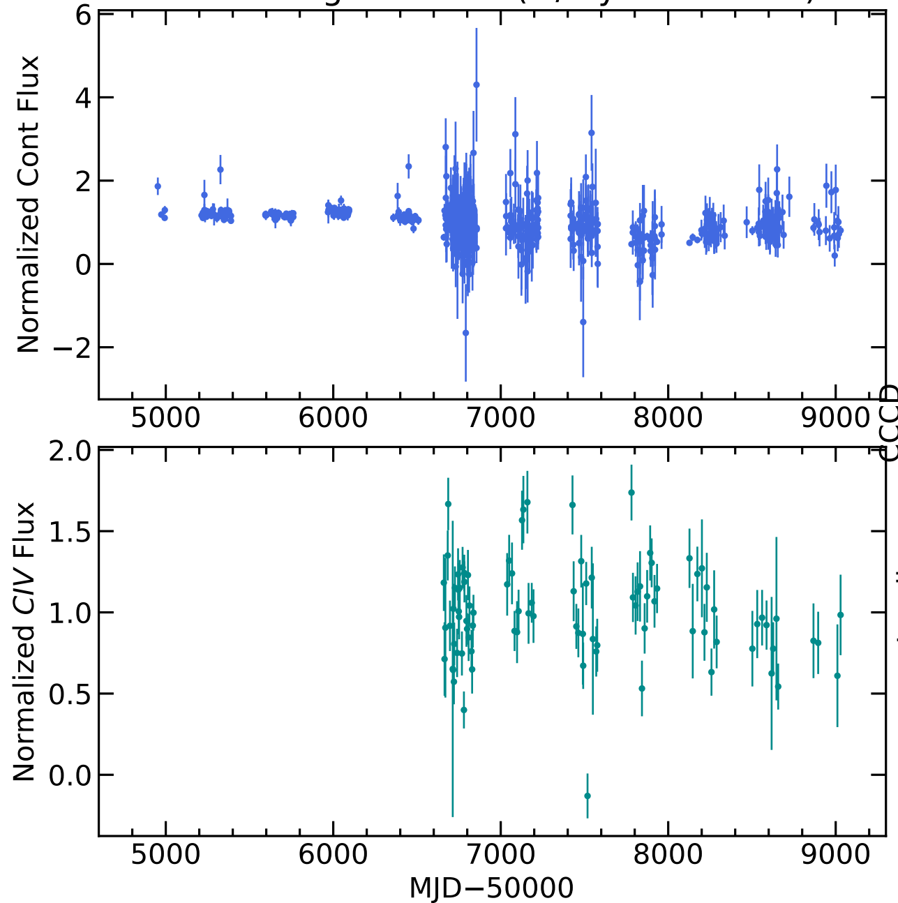
RM476 Light Curves (w/ PyROA model)
