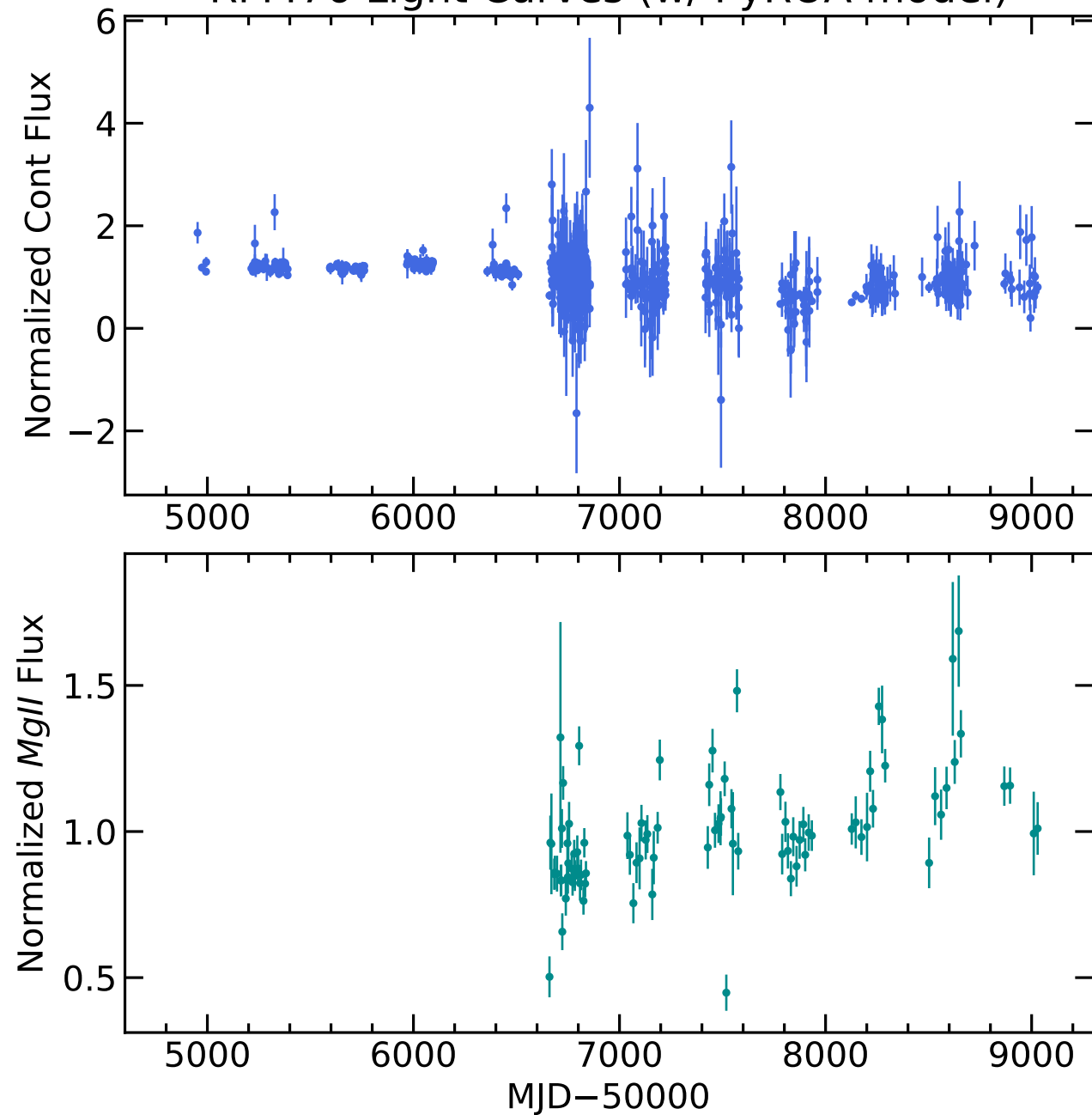
RM476 Light Curves (w/ PyROA model)
