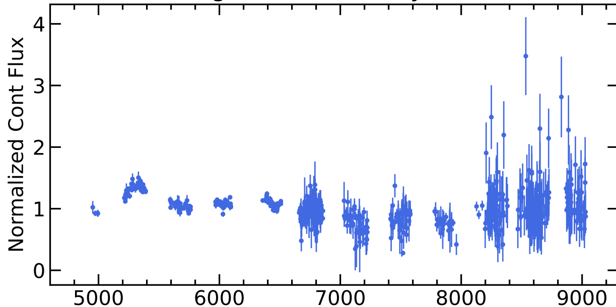
RM477 Light Curves (w/ PyROA model)
