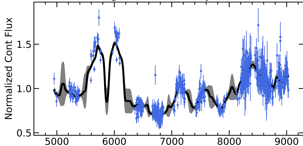
RM478 Light Curves (w/ PyROA model)
