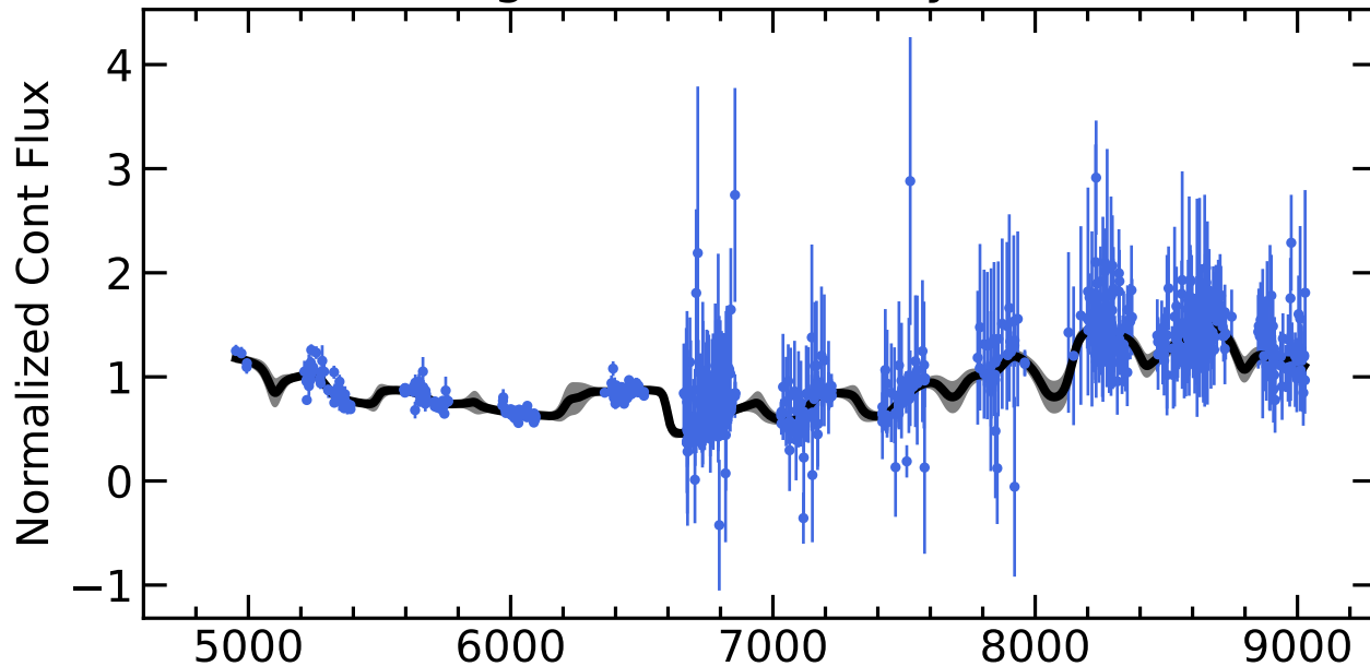
RM479 Light Curves (w/ PyROA model)
