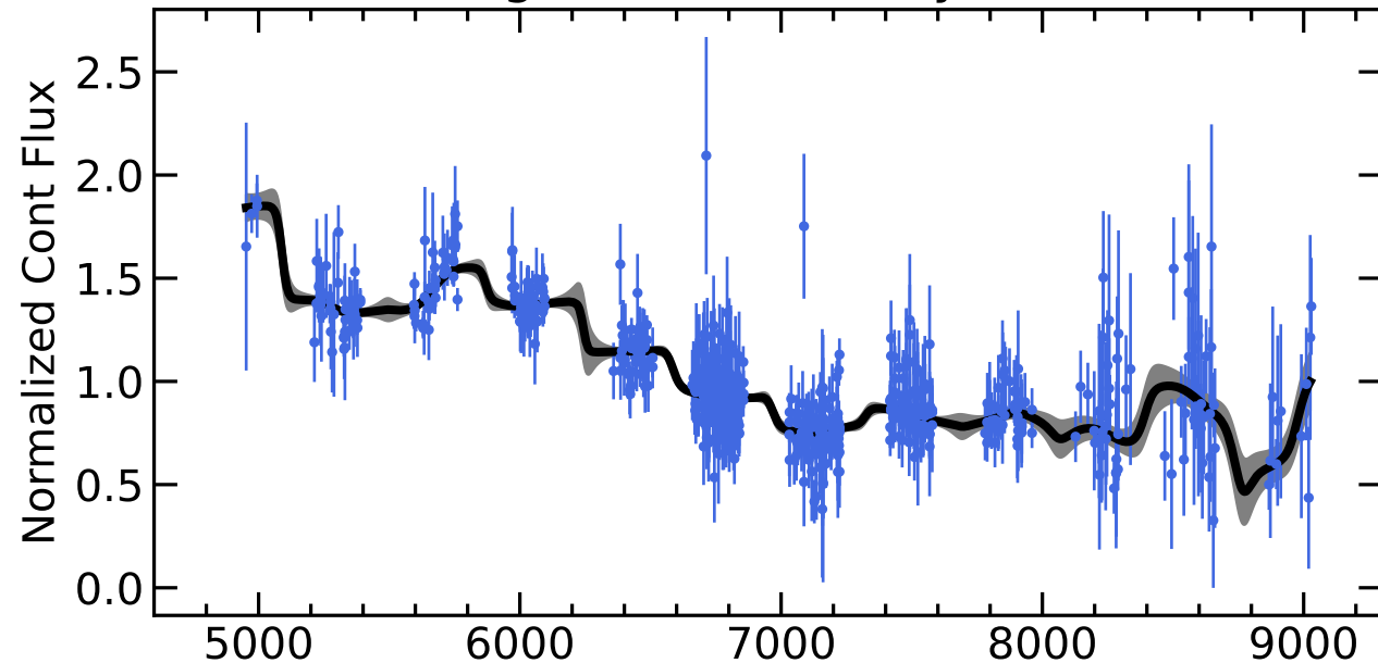
RM480 Light Curves (w/ PyROA model)
