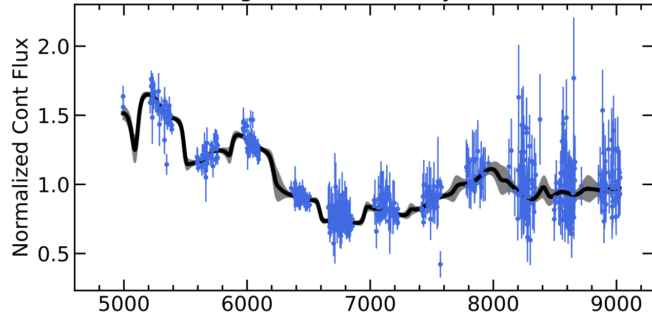
RM481 Light Curves (w/ PyROA model)
