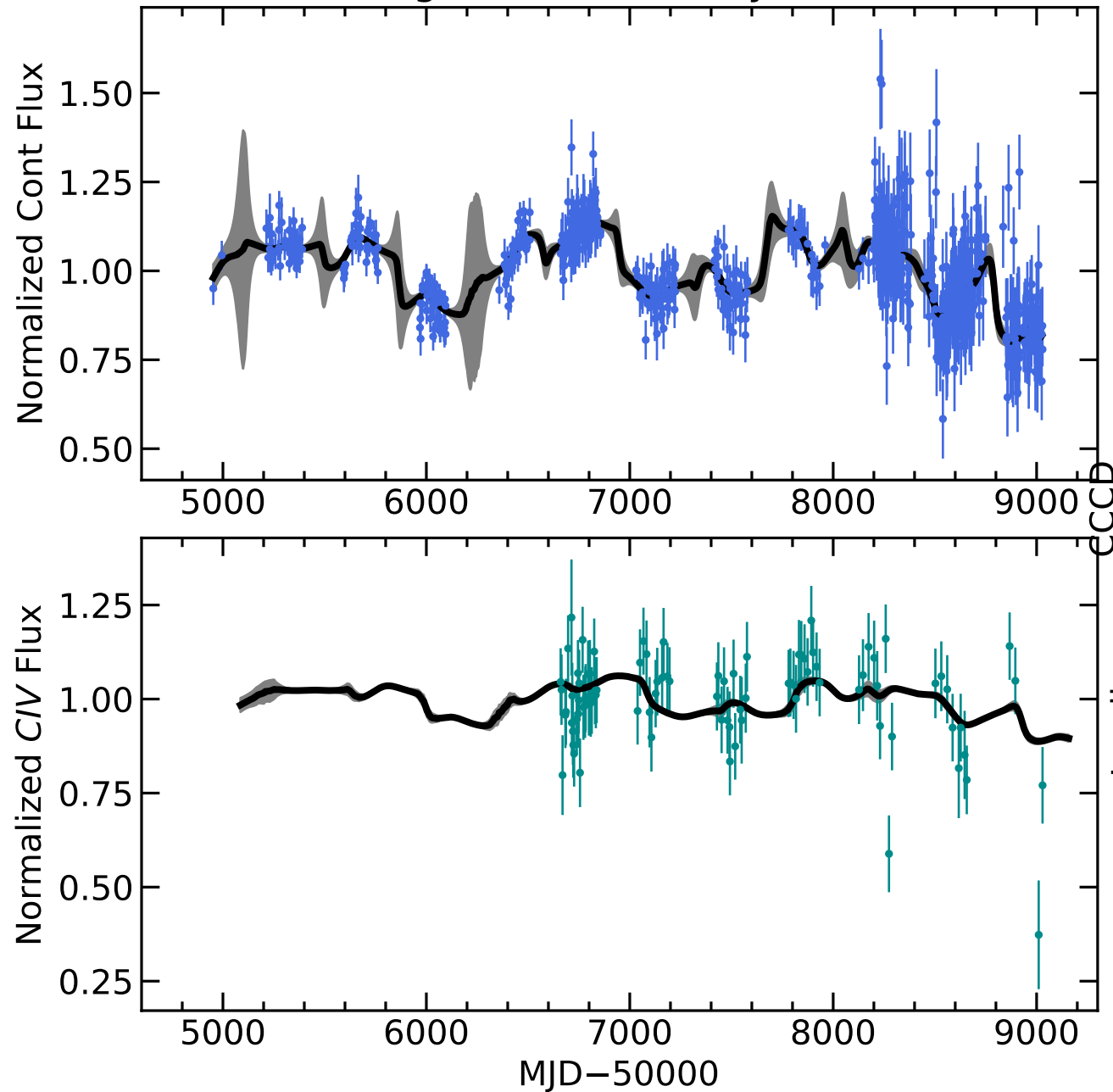
RM482 Light Curves (w/ PyROA model)
