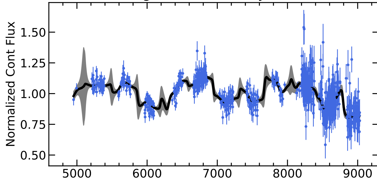
RM482 Light Curves (w/ PyROA model)
