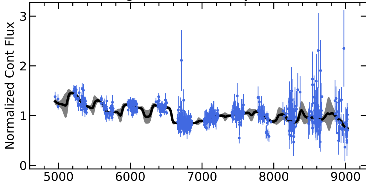
RM483 Light Curves (w/ PyROA model)
