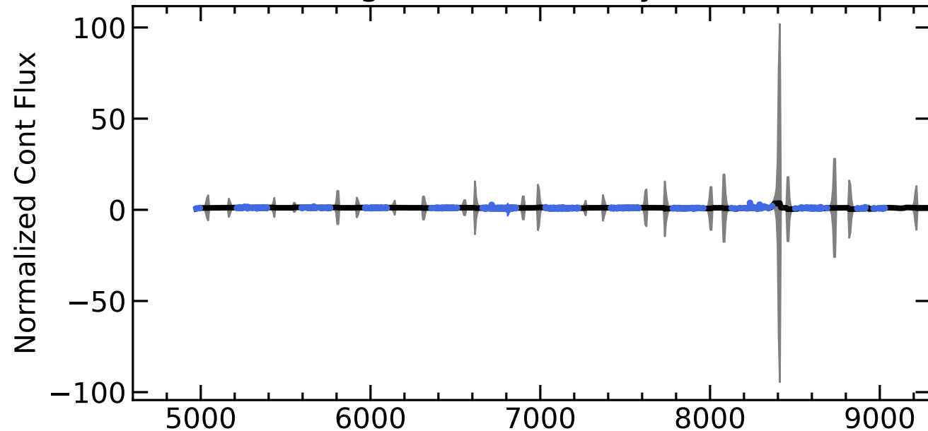
RM484 Light Curves (w/ PyROA model)
