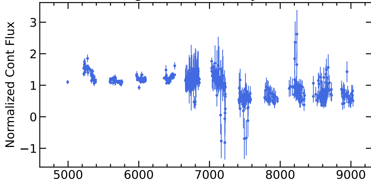
RM487 Light Curves (w/ PyROA model)
