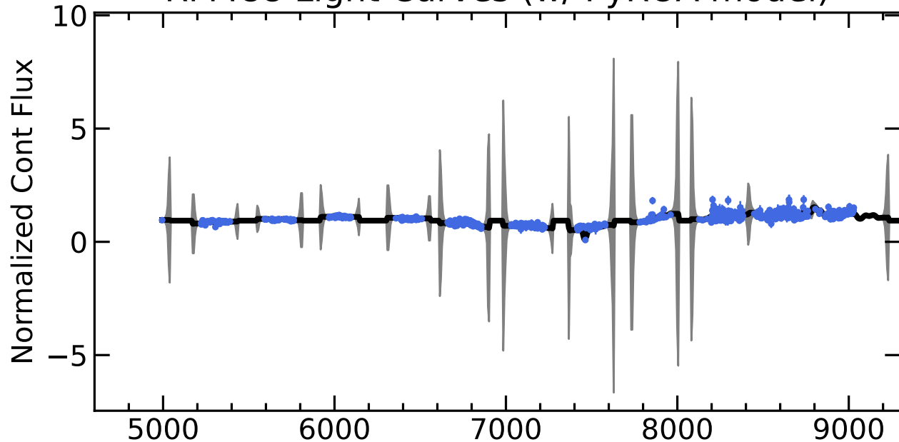
RM488 Light Curves (w/ PyROA model)
