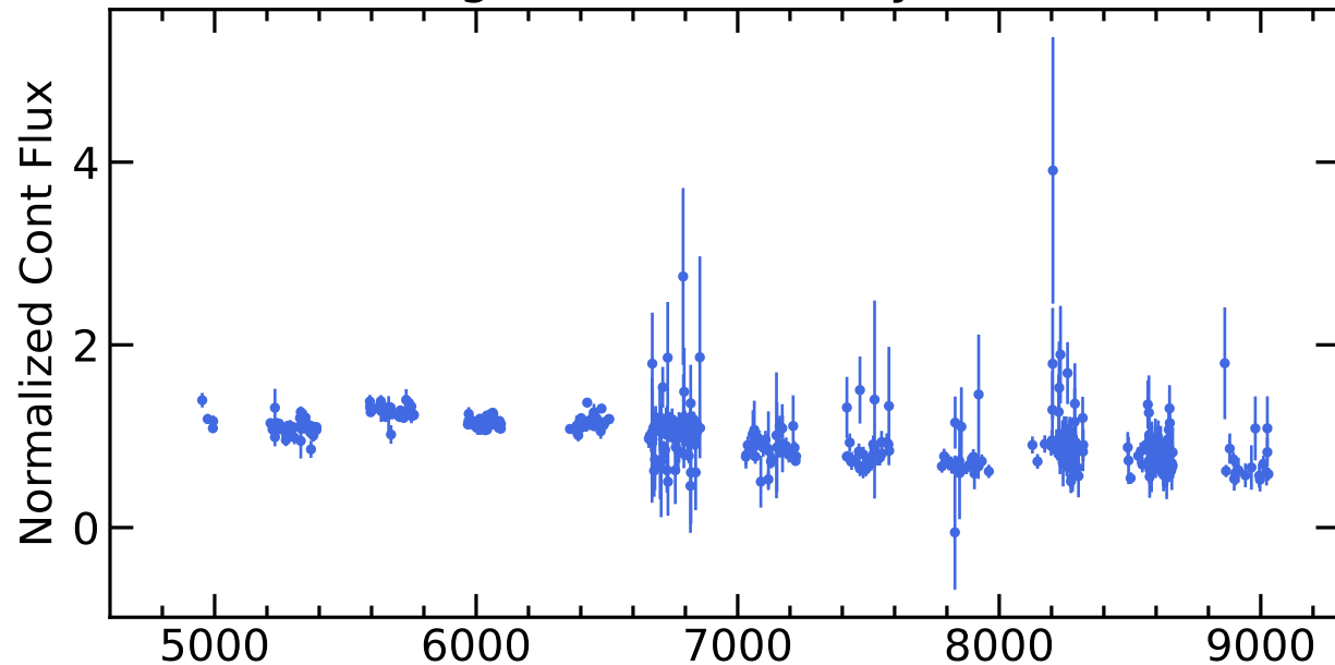
RM489 Light Curves (w/ PyROA model)
