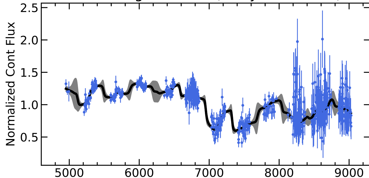
RM490 Light Curves (w/ PyROA model)
