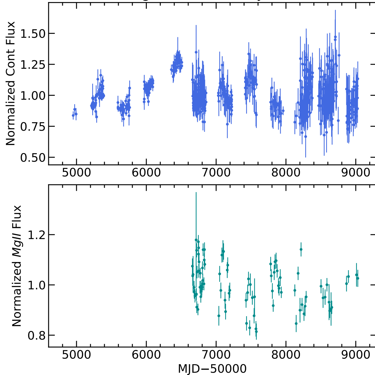
RM491 Light Curves (w/ PyROA model)
