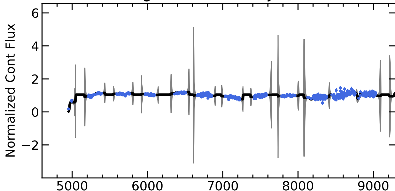
RM492 Light Curves (w/ PyROA model)
