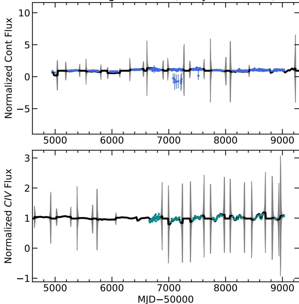
RM493 Light Curves (w/ PyROA model)
