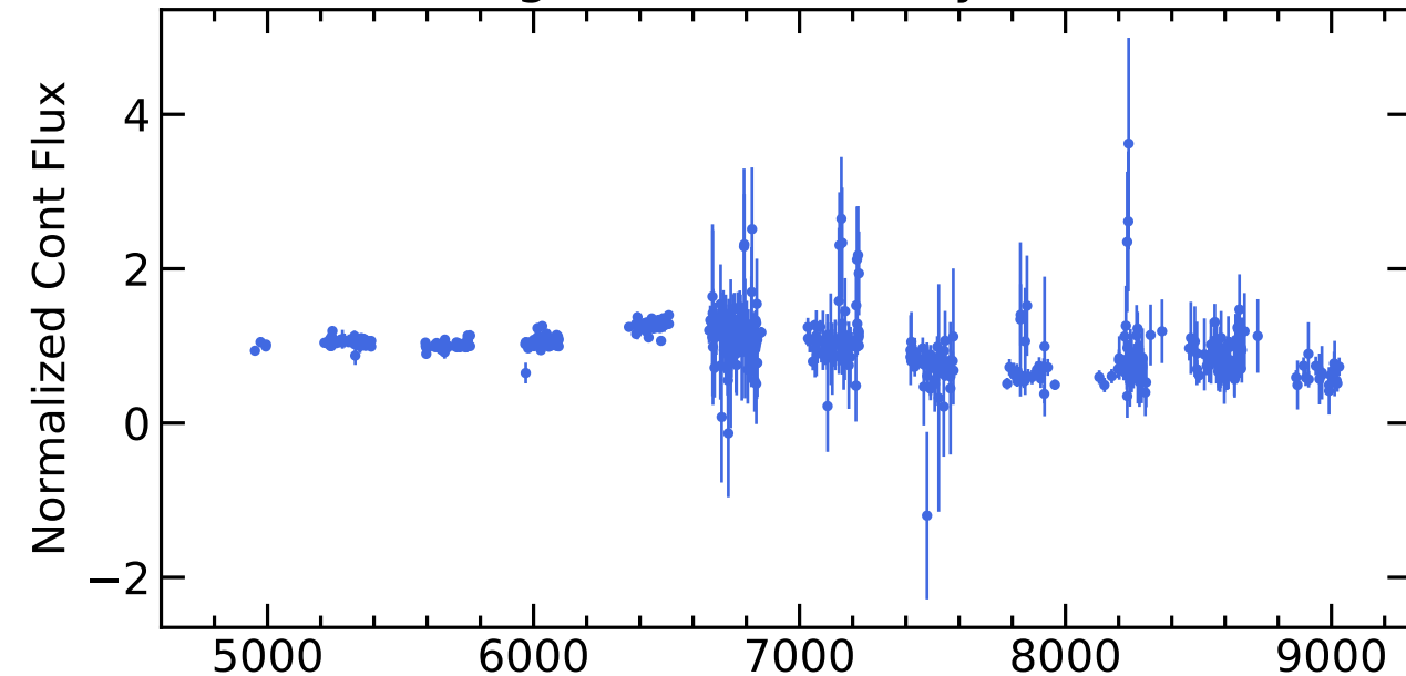
RM494 Light Curves (w/ PyROA model)
