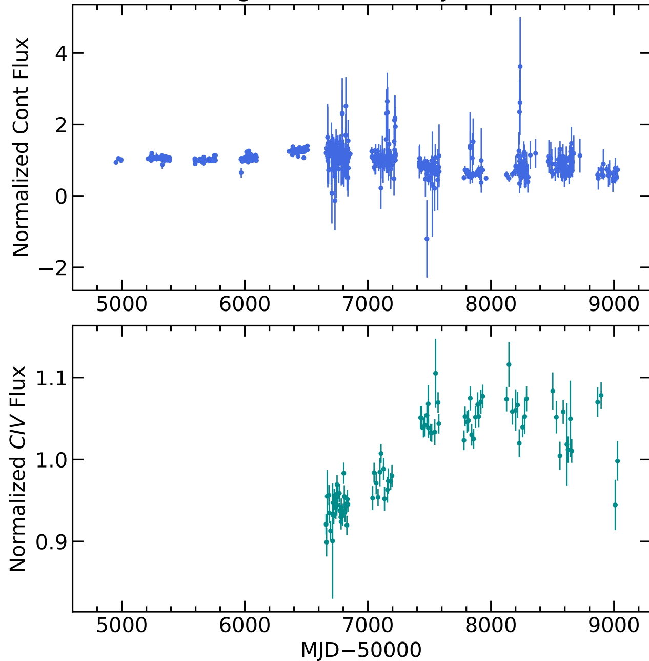
RM494 Light Curves (w/ PyROA model)
