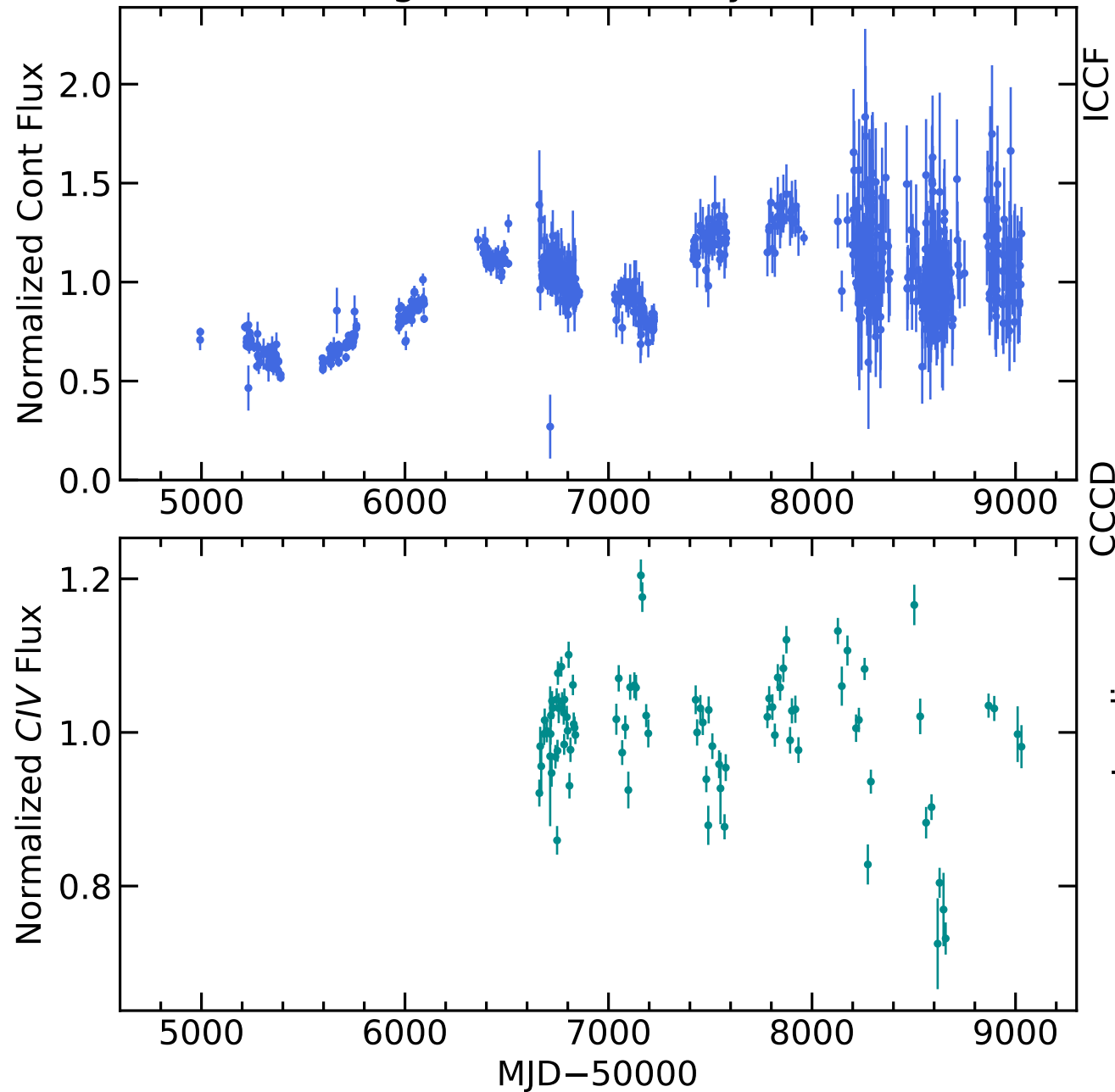
RM495 Light Curves (w/ PyROA model)
