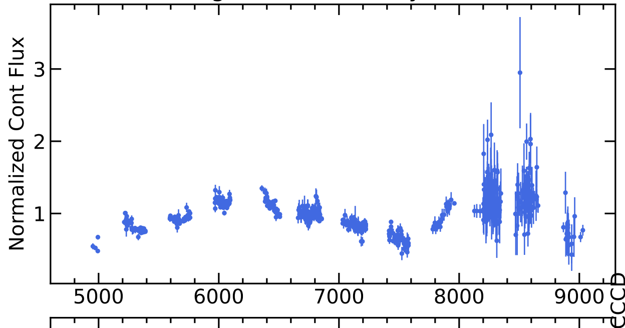
RM496 Light Curves (w/ PyROA model)
