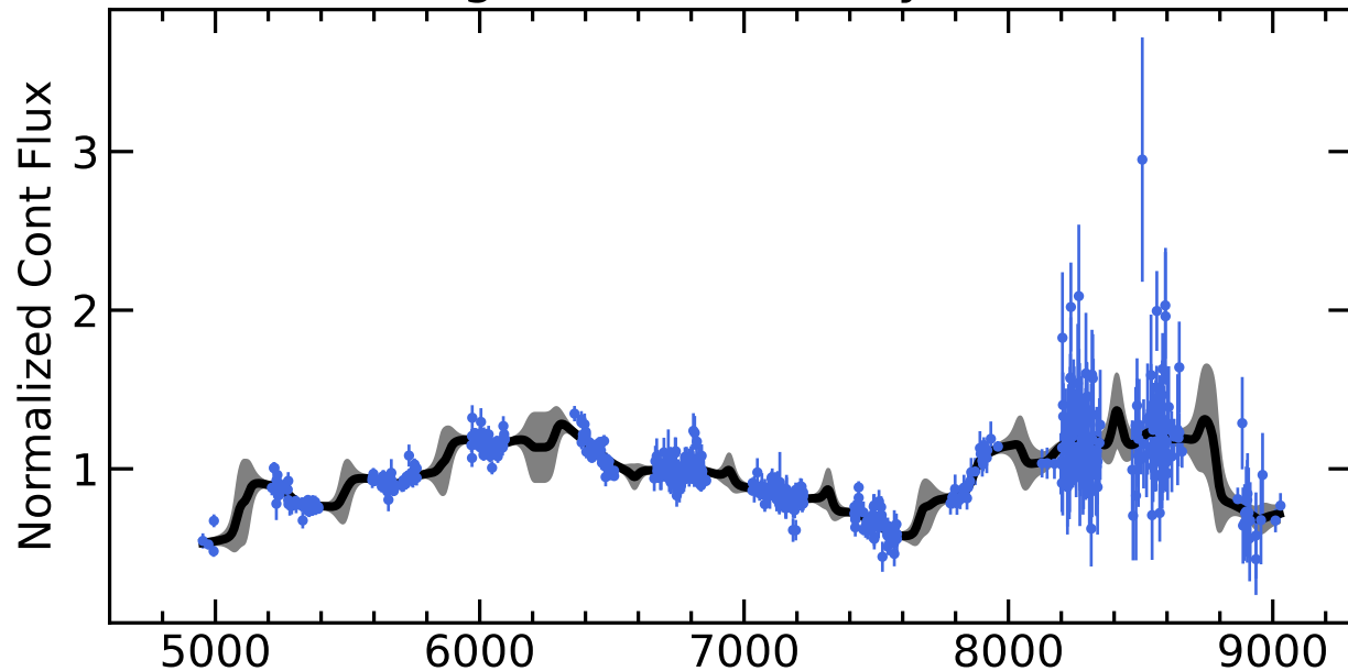
RM496 Light Curves (w/ PyROA model)
