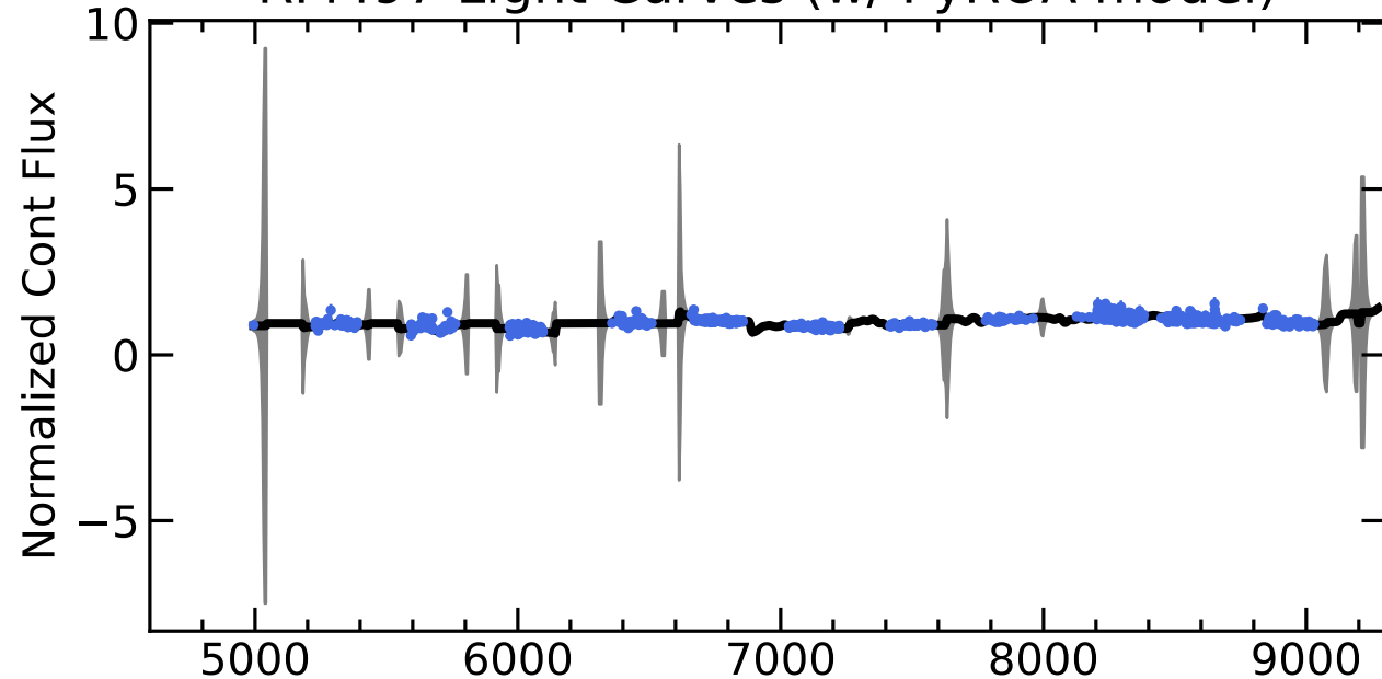
RM497 Light Curves (w/ PyROA model)
