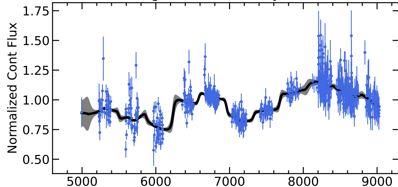
RM497 Light Curves (w/ PyROA model)
