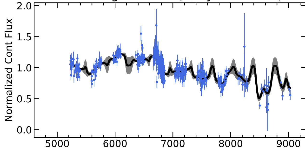
RM498 Light Curves (w/ PyROA model)
