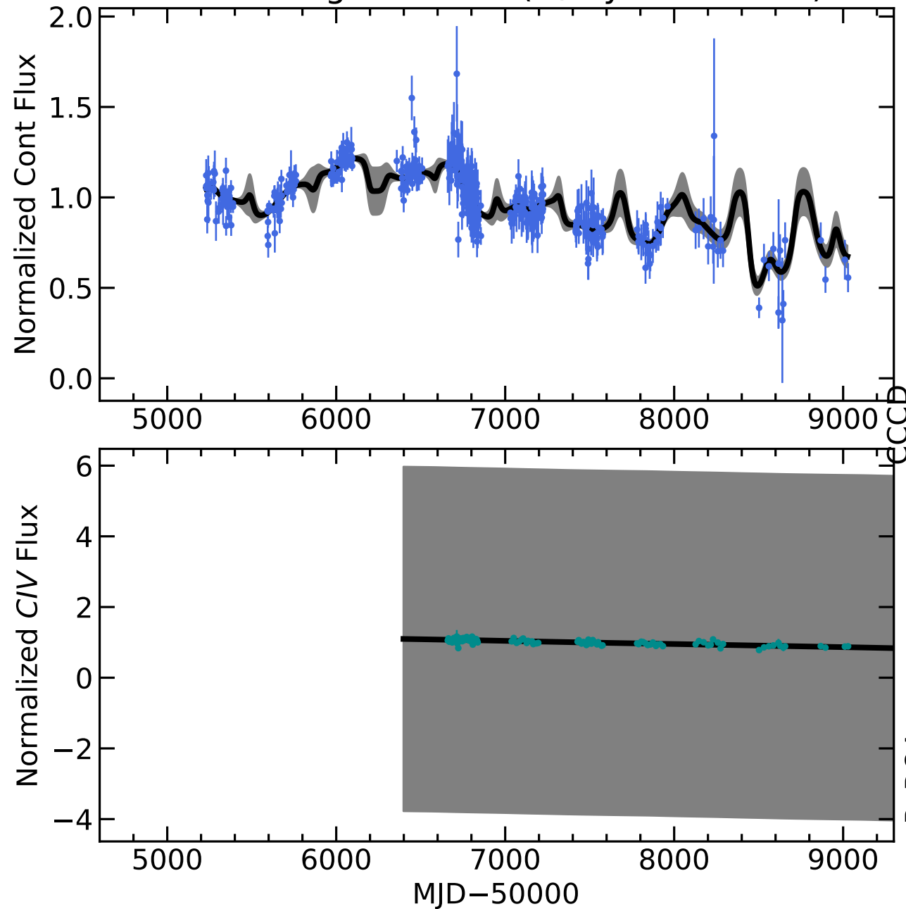
RM498 Light Curves (w/ PyROA model)
