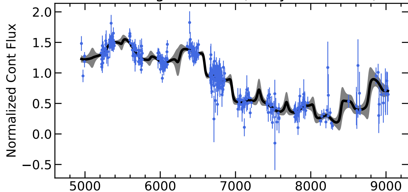
RM499 Light Curves (w/ PyROA model)
