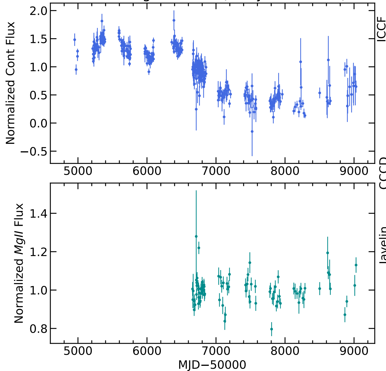
RM499 Light Curves (w/ PyROA model)
