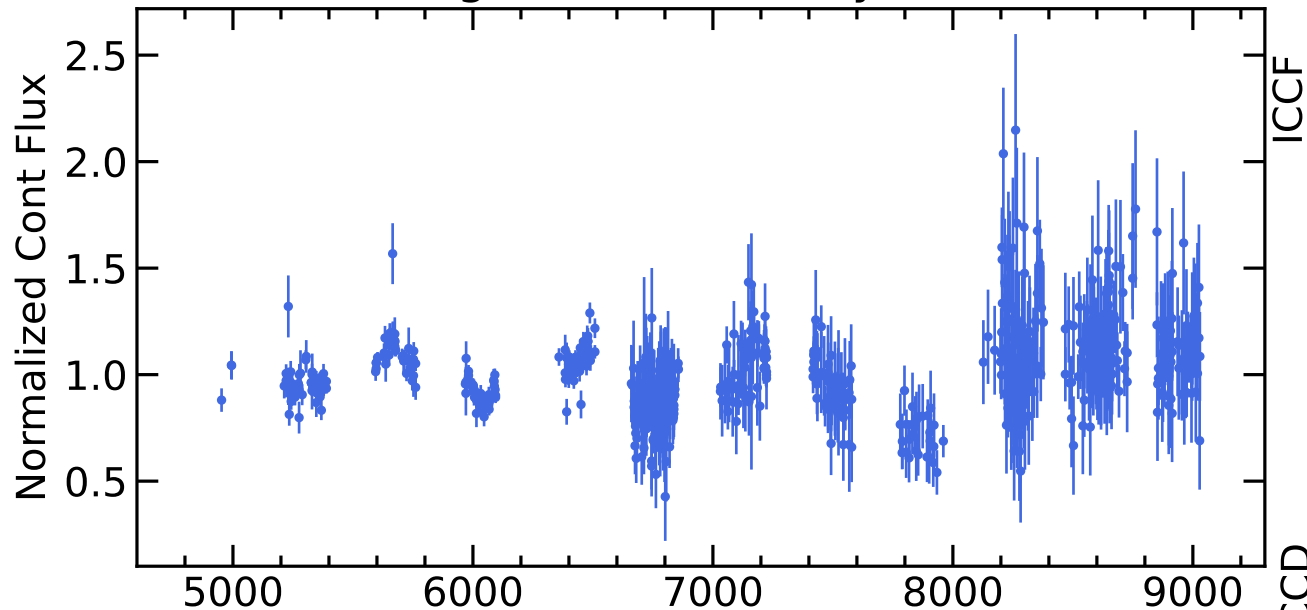
RM500 Light Curves (w/ PyROA model)
