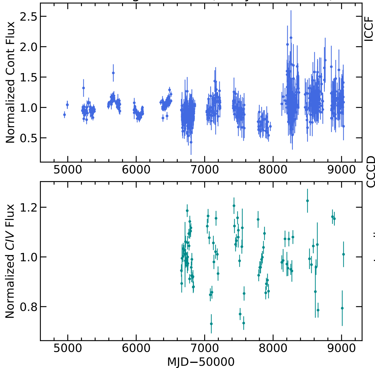
RM500 Light Curves (w/ PyROA model)
