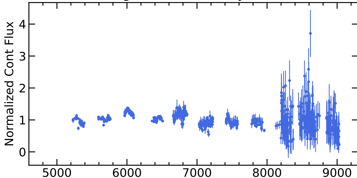
RM501 Light Curves (w/ PyROA model)
