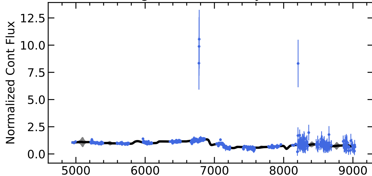
RM502 Light Curves (w/ PyROA model)
