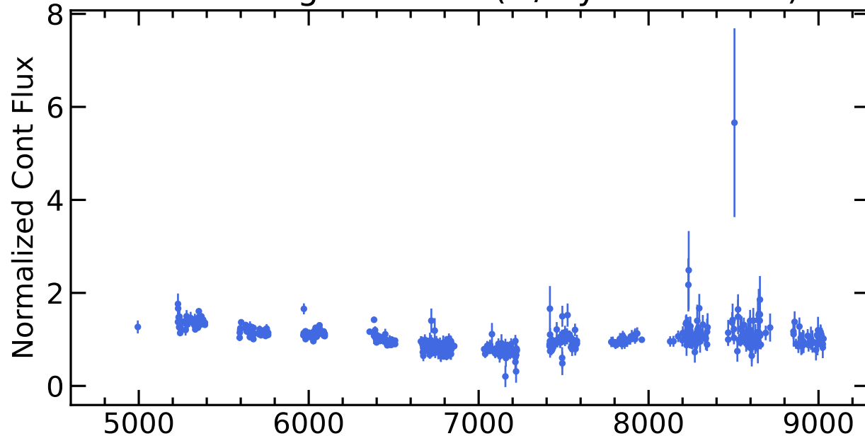
RM504 Light Curves (w/ PyROA model)
