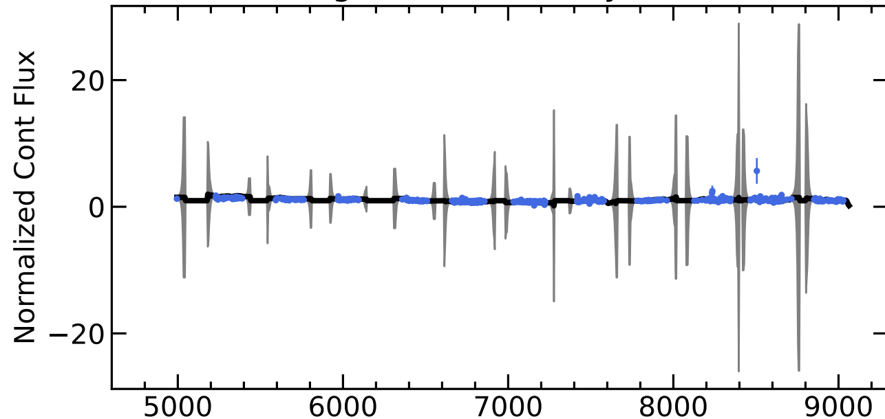
RM504 Light Curves (w/ PyROA model)
