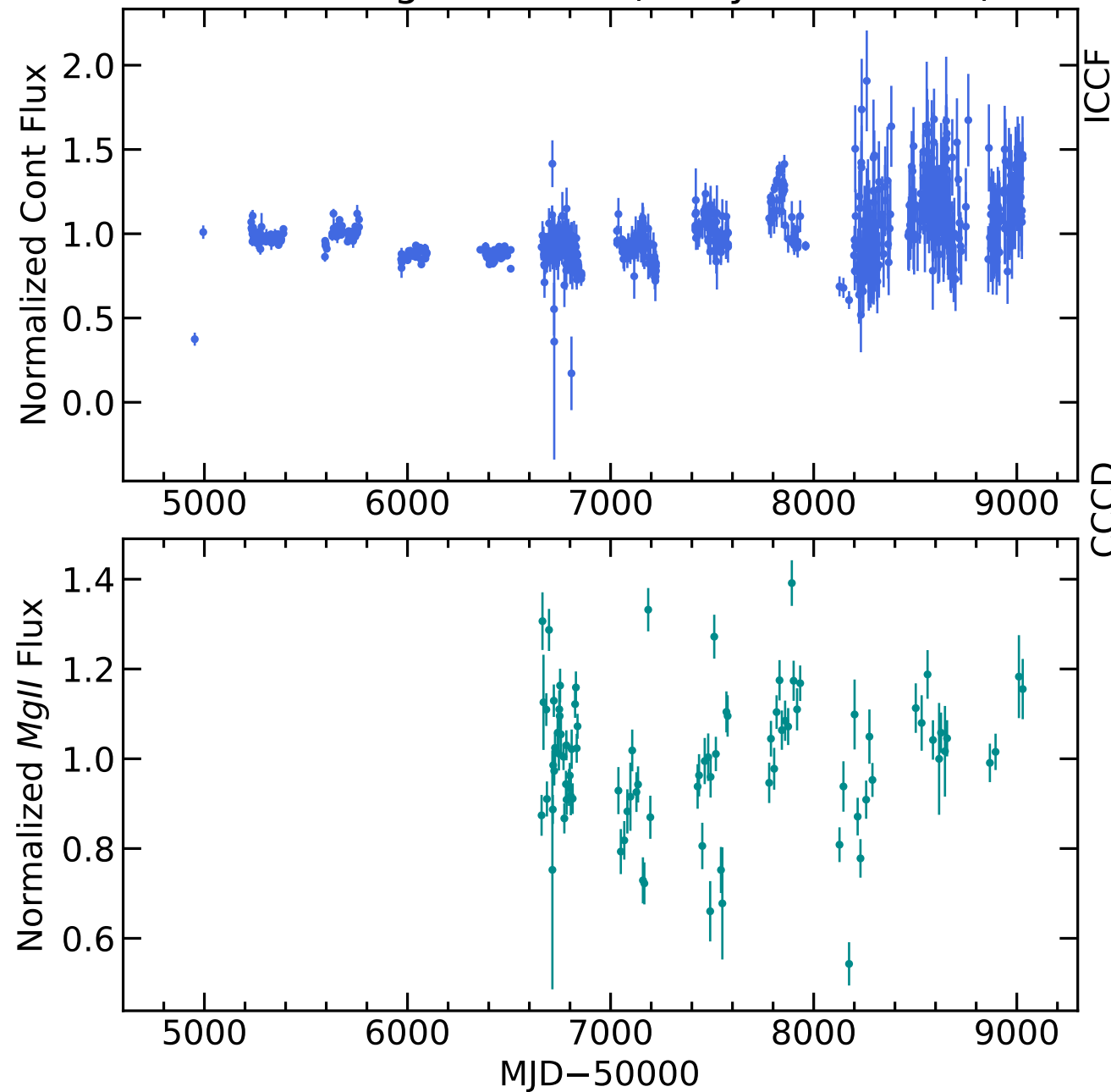
RM505 Light Curves (w/ PyROA model)
