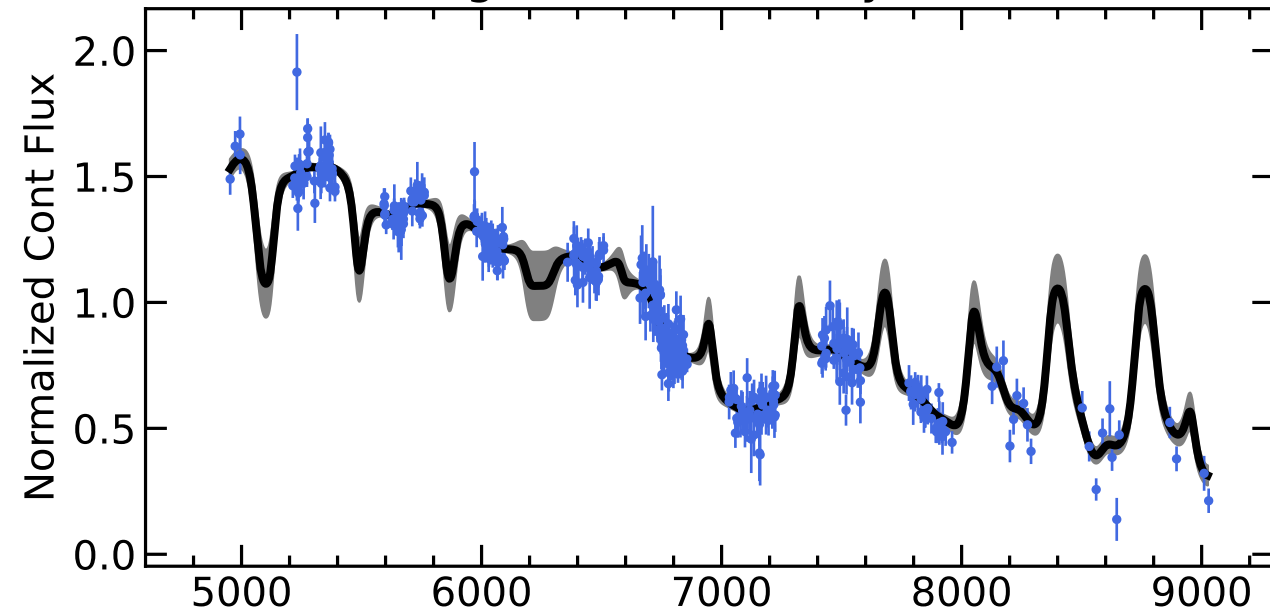
RM506 Light Curves (w/ PyROA model)
