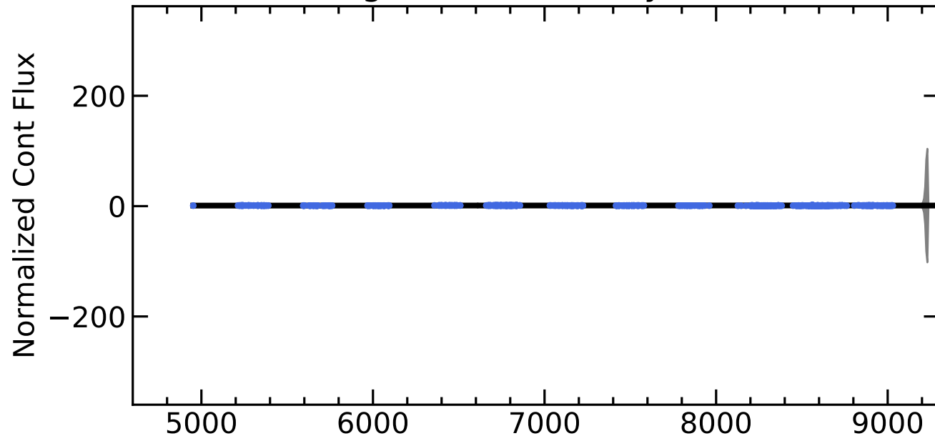
RM507 Light Curves (w/ PyROA model)
