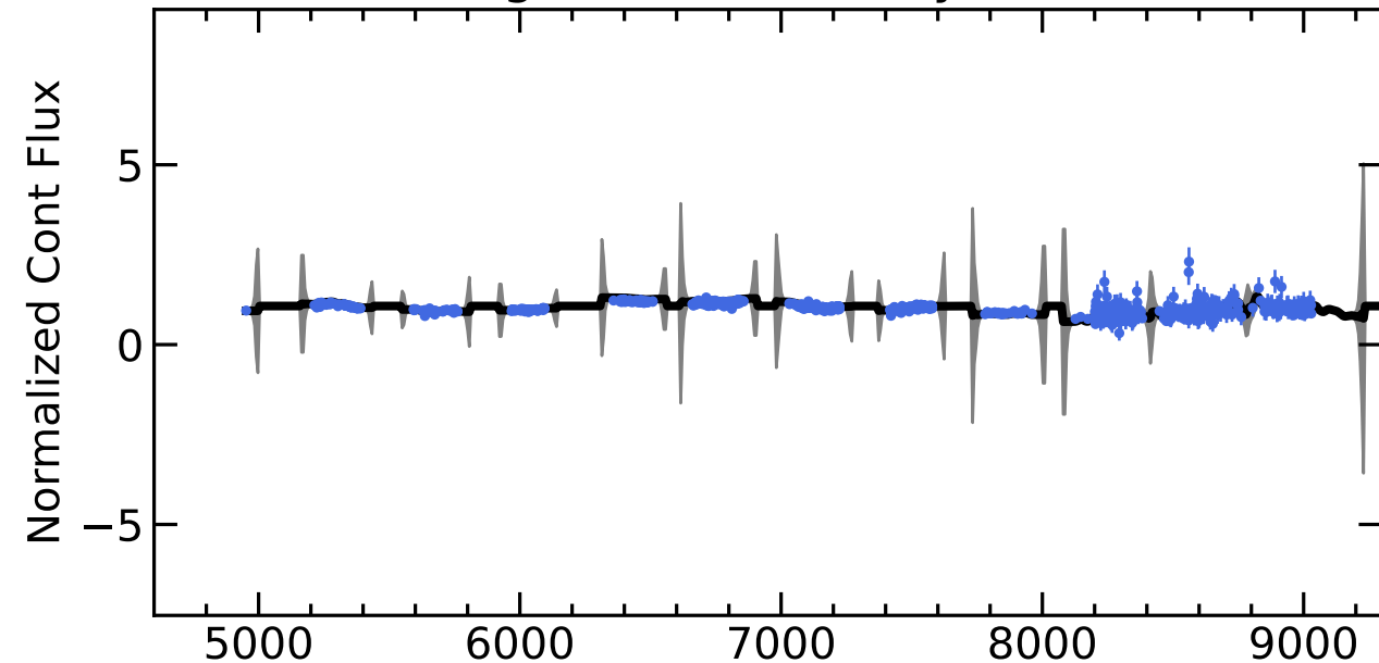
RM507 Light Curves (w/ PyROA model)
