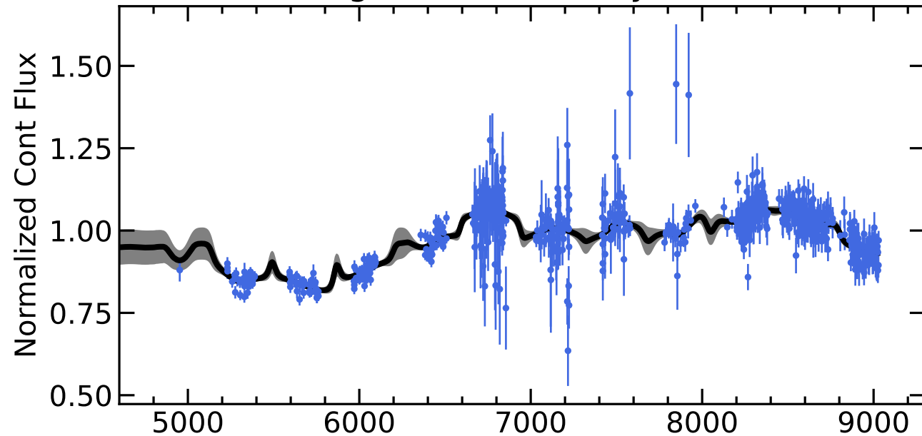
RM508 Light Curves (w/ PyROA model)
