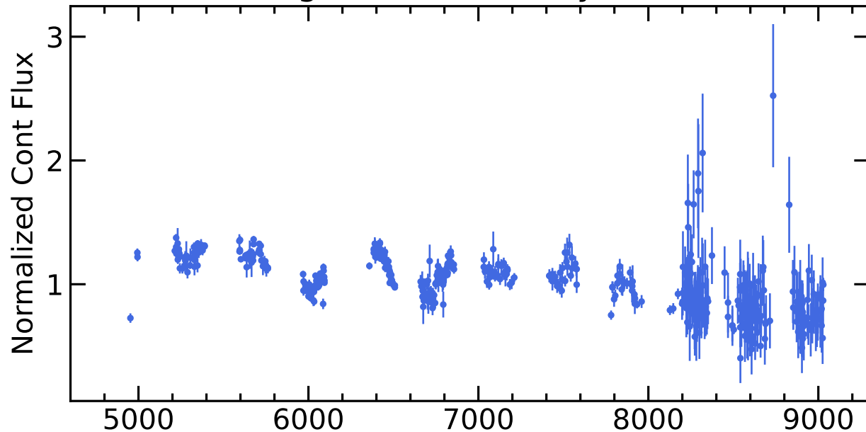
RM510 Light Curves (w/ PyROA model)
