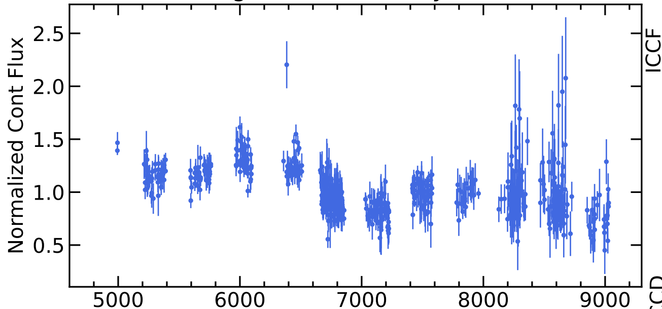
RM511 Light Curves (w/ PyROA model)
