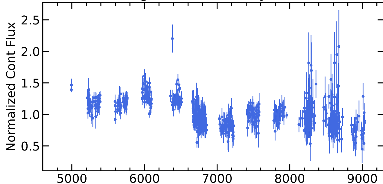
RM511 Light Curves (w/ PyROA model)
