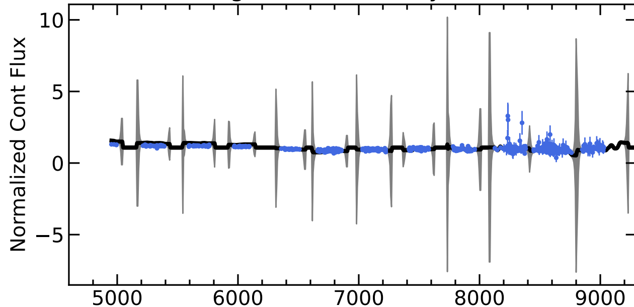
RM512 Light Curves (w/ PyROA model)
