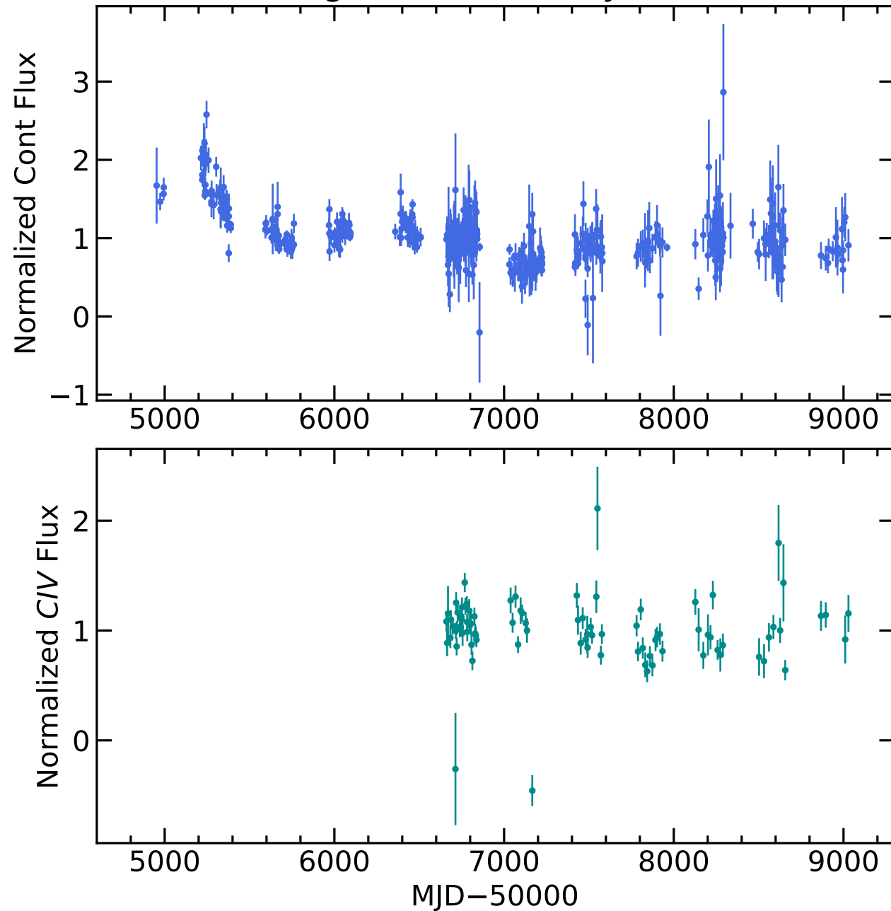
RM513 Light Curves (w/ PyROA model)
