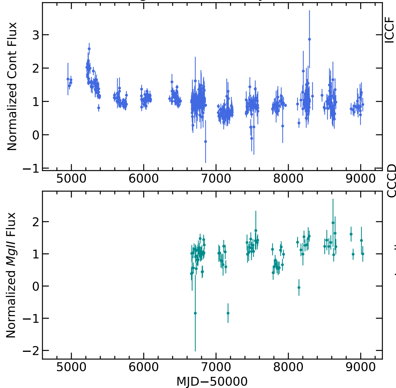
RM513 Light Curves (w/ PyROA model)
