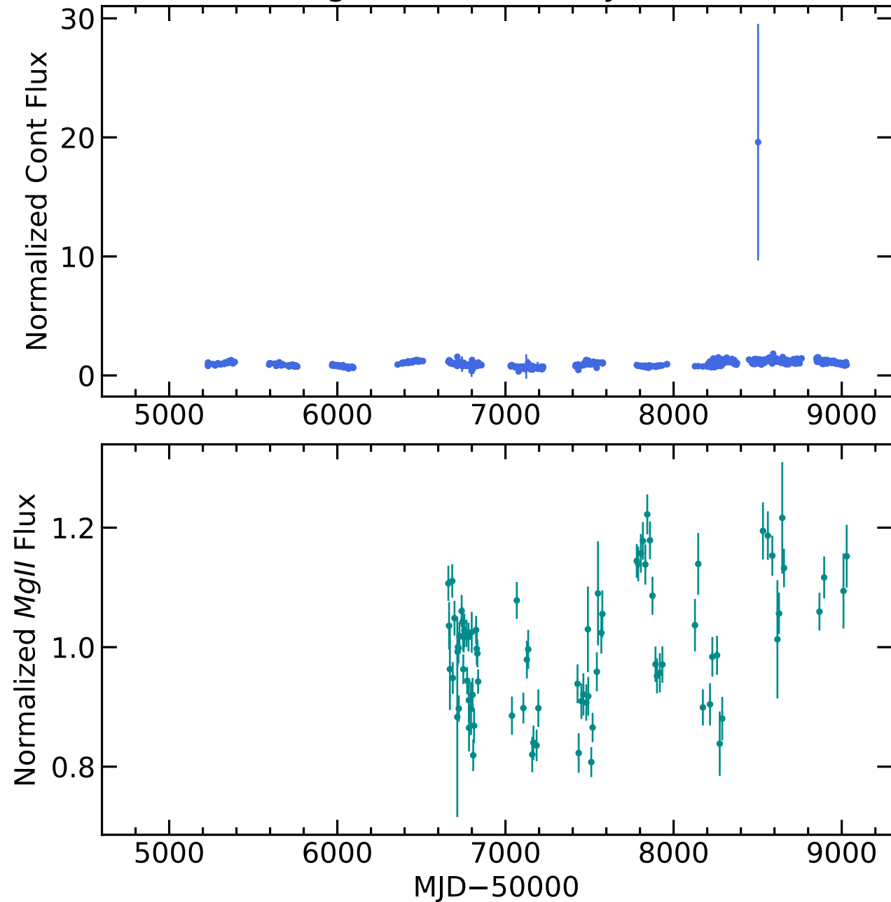
RM515 Light Curves (w/ PyROA model)
