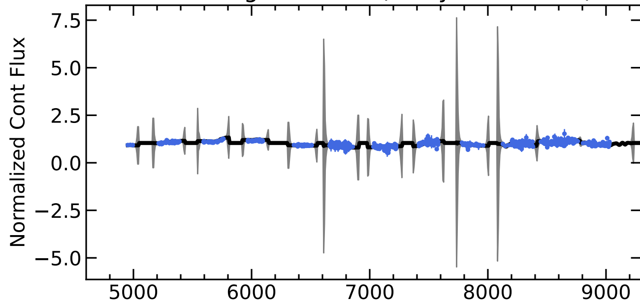
RM517 Light Curves (w/ PyROA model)
