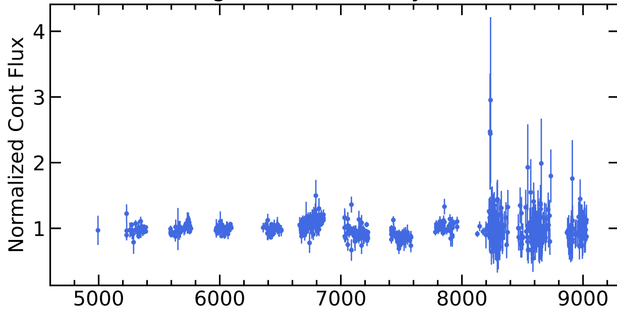
RM518 Light Curves (w/ PyROA model)
