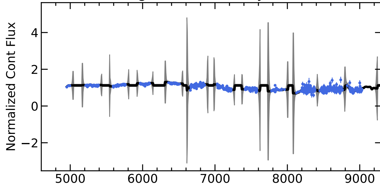
RM520 Light Curves (w/ PyROA model)
