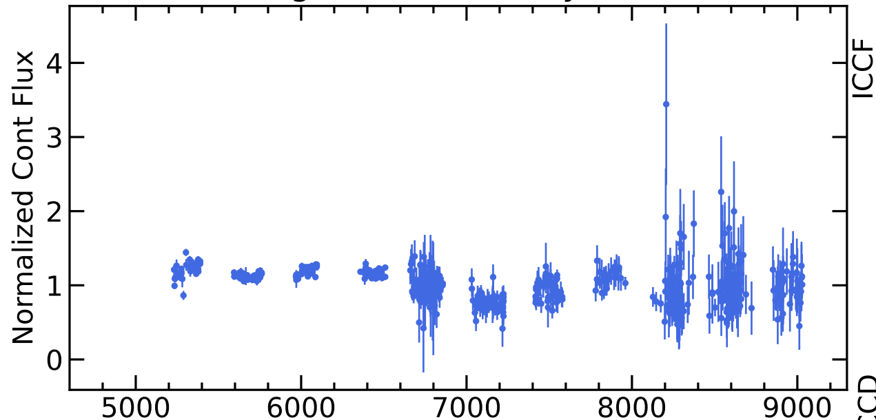
RM521 Light Curves (w/ PyROA model)
