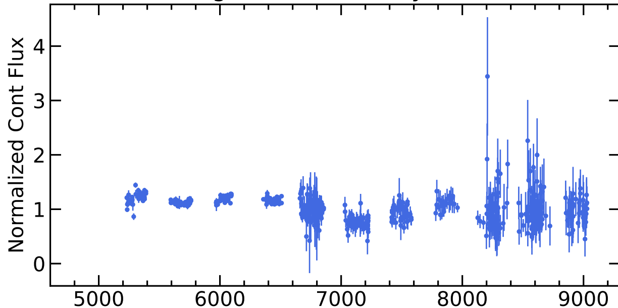
RM521 Light Curves (w/ PyROA model)
