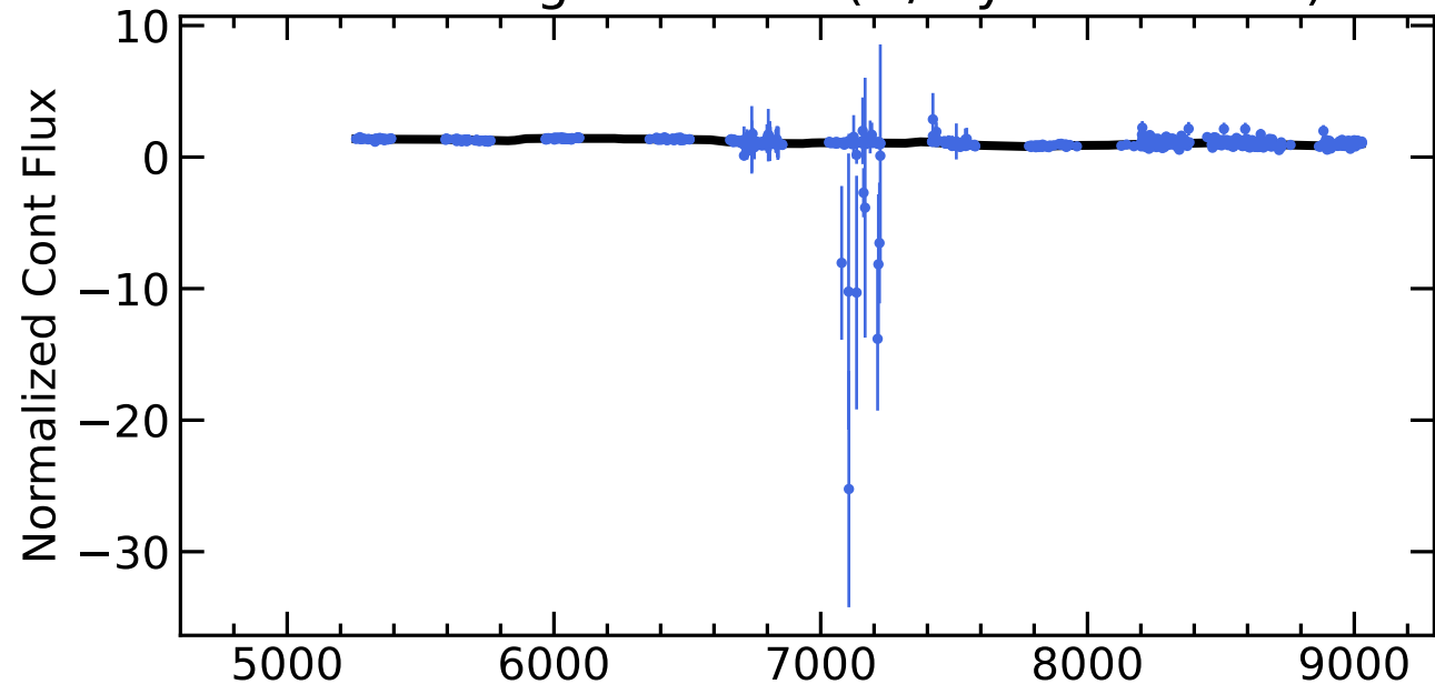
RM522 Light Curves (w/ PyROA model)
