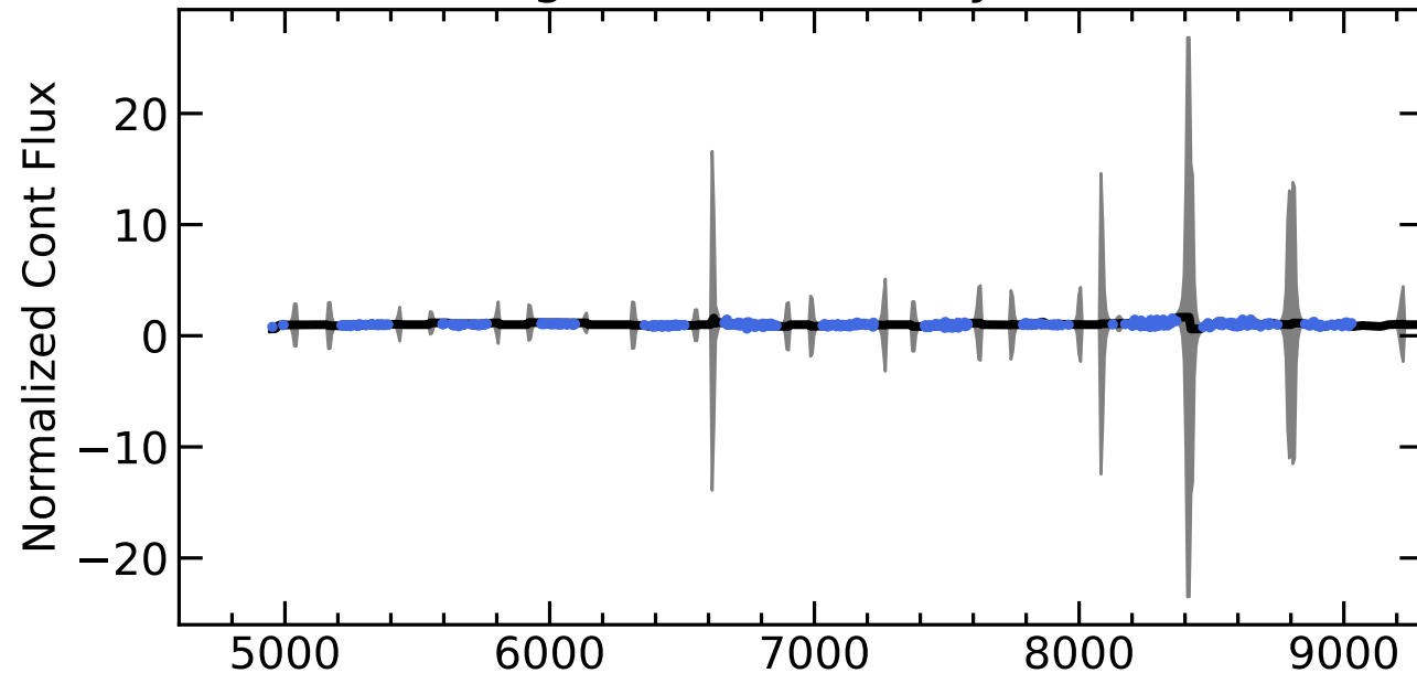
RM526 Light Curves (w/ PyROA model)
