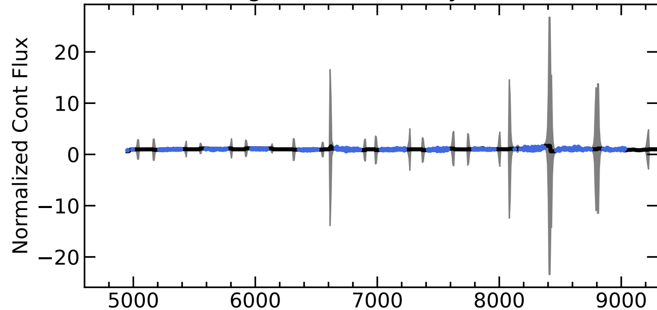
RM526 Light Curves (w/ PyROA model)
