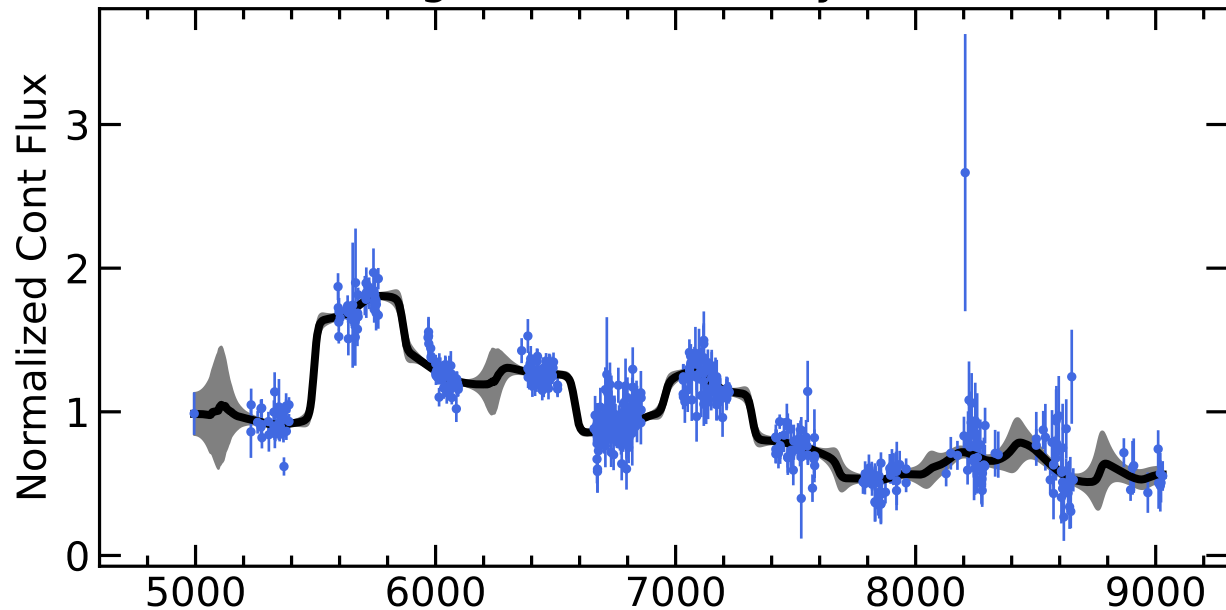
RM527 Light Curves (w/ PyROA model)
