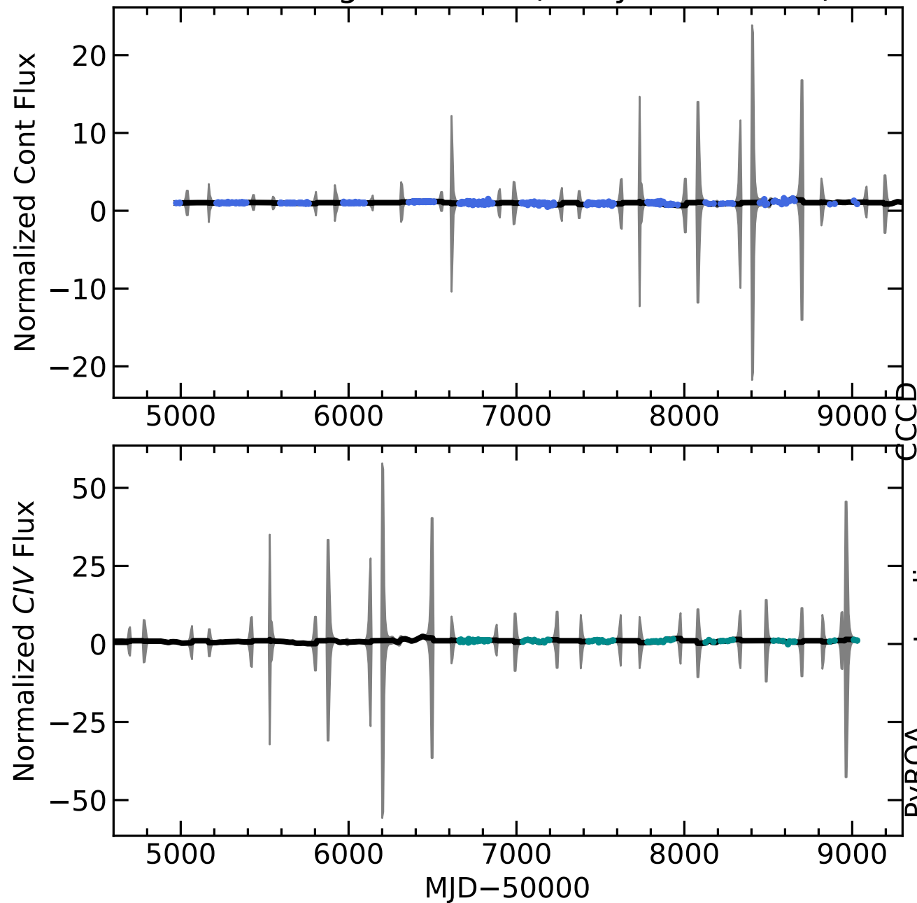
RM528 Light Curves (w/ PyROA model)
