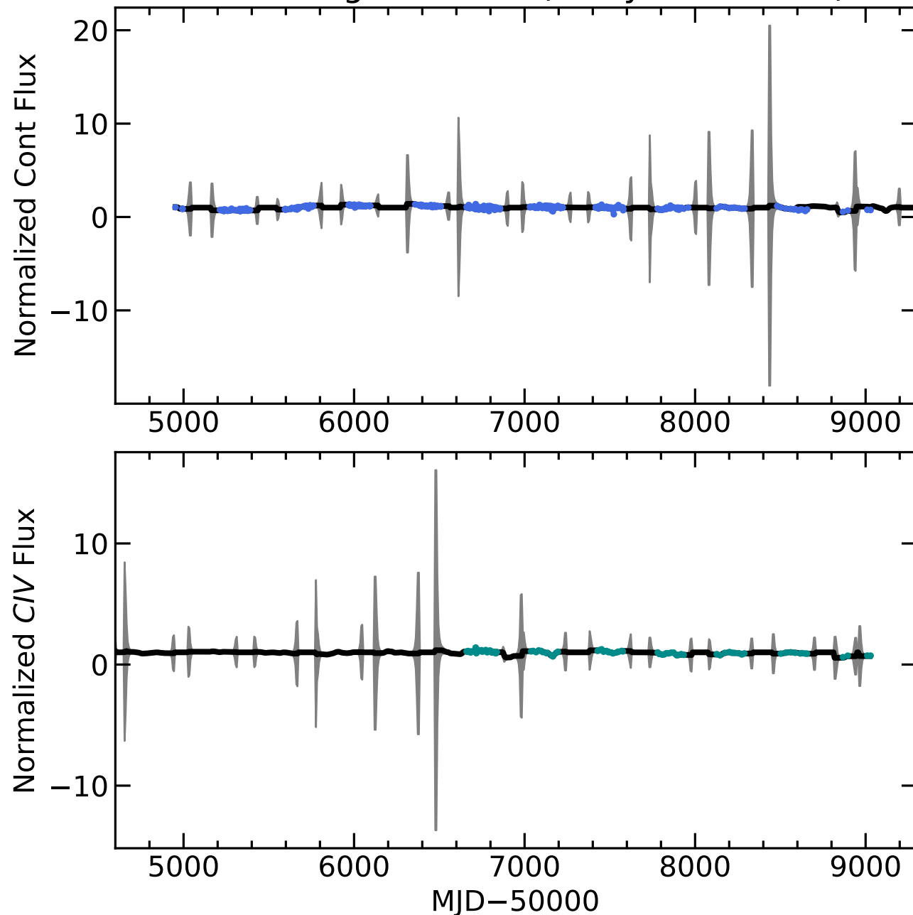
RM529 Light Curves (w/ PyROA model)
