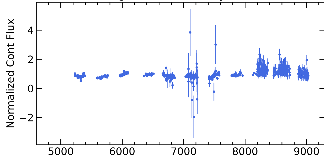
RM530 Light Curves (w/ PyROA model)
