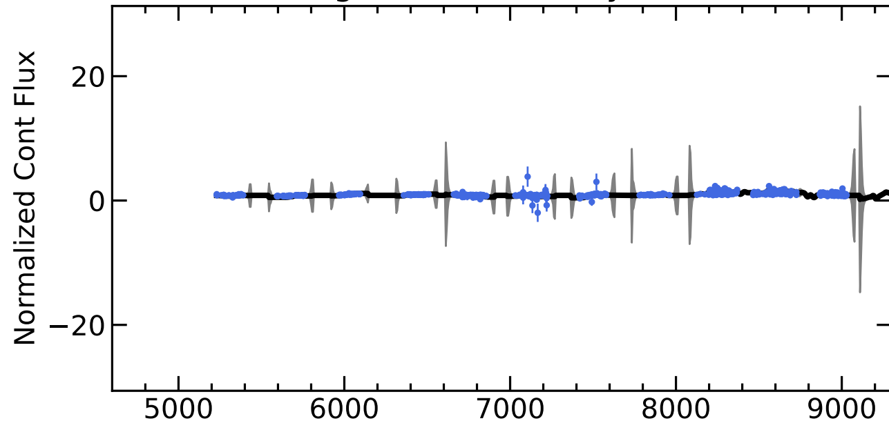
RM530 Light Curves (w/ PyROA model)
