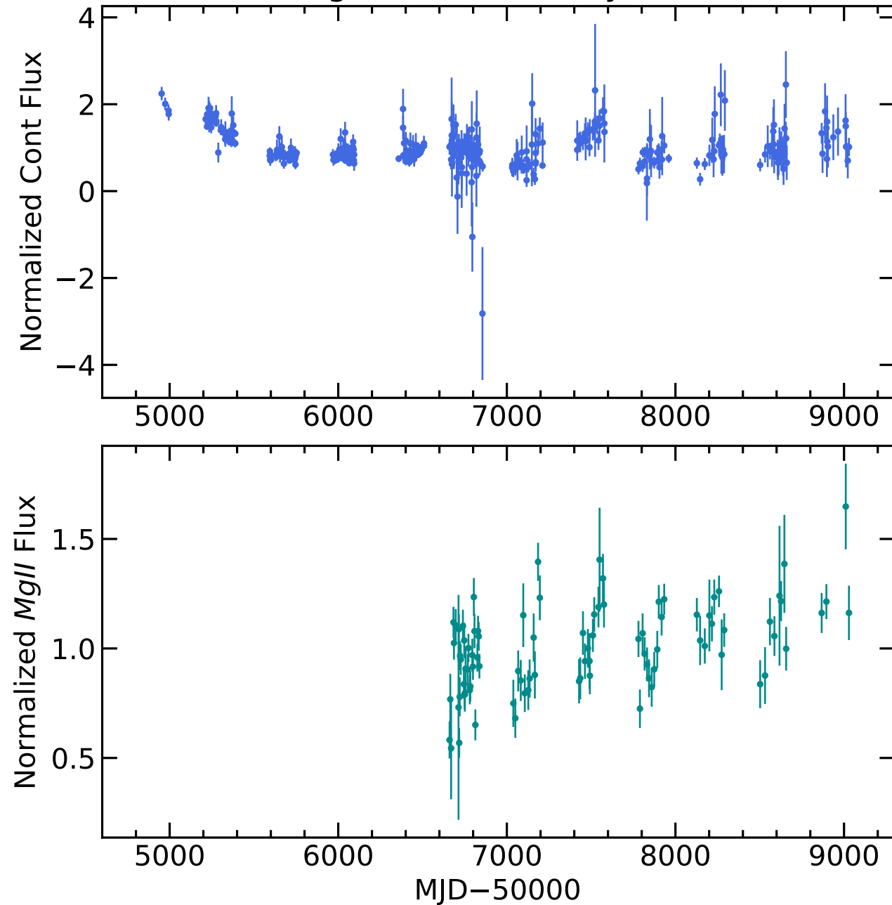
RM531 Light Curves (w/ PyROA model)
